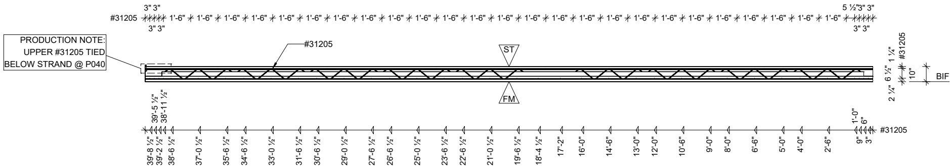
SECTION VIEW
