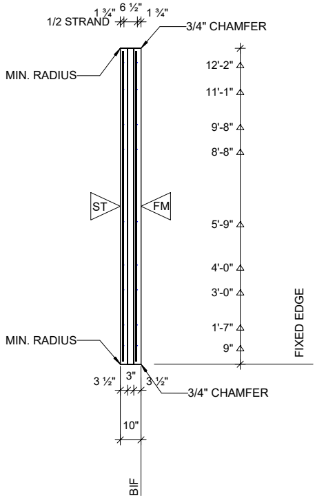
SECTION VIEW
