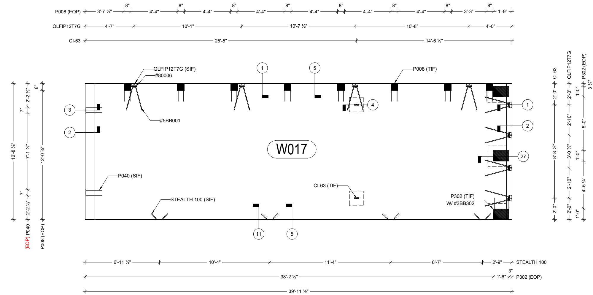
FORM VIEW
